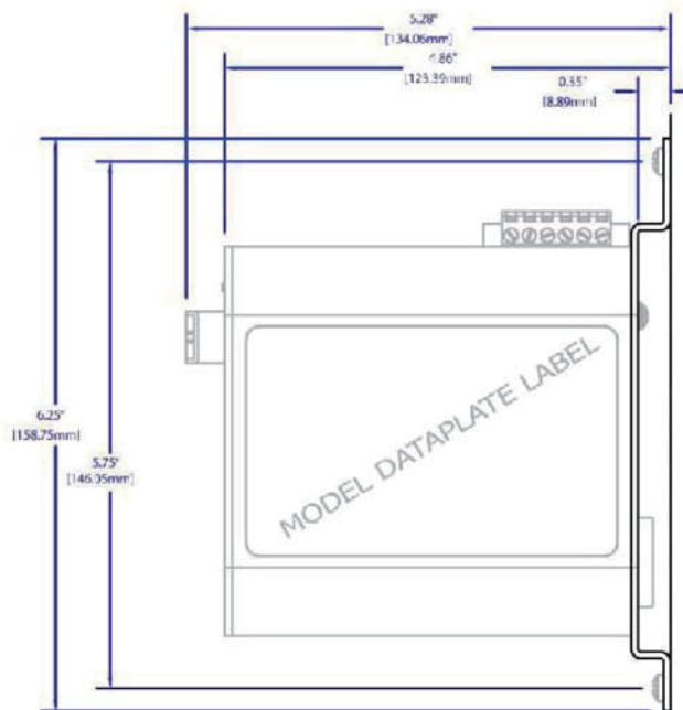
OPTIONAL COMPACT PANEL MOUNT ASSY. ( P/N: CPMA-1 )
